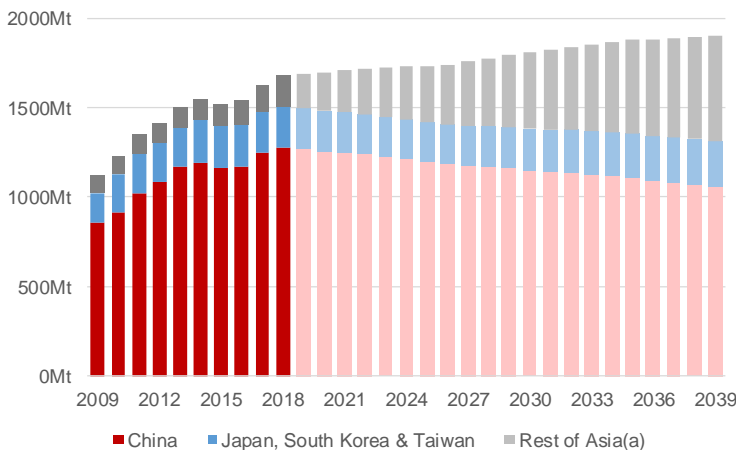
1 Dry million tonnes. (a) India, Vietnam, Malaysia, Indonesia, Philippines and other Asian countries. Source: AME, Iron Ore Strategic Studies (Quarterly).
