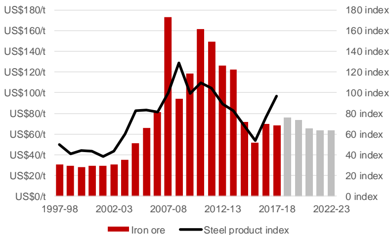
1 China spot price in nominal US dollars, cost and freight (CFR). 2 China steel product price index (2007-08 = 100.0). Source: World Bank, Commodity Markets; CEIC, China Premium Database; and 3 WA Government 2019-20 State Budget.
